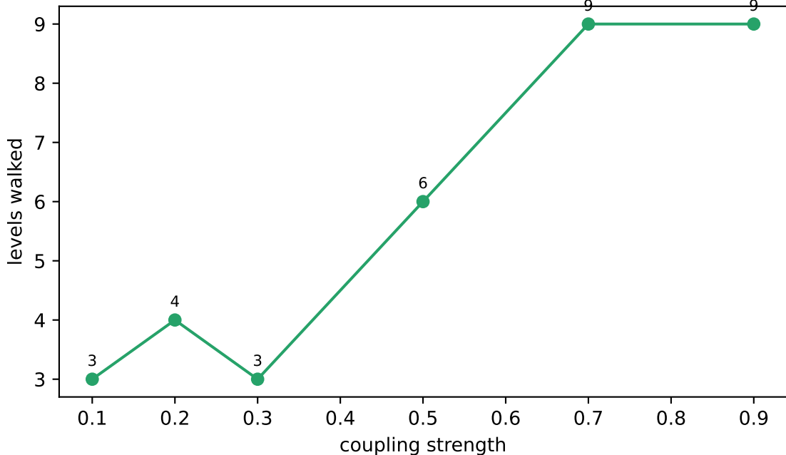
Walk depth scales with signal (priced-stop budget allocation)
