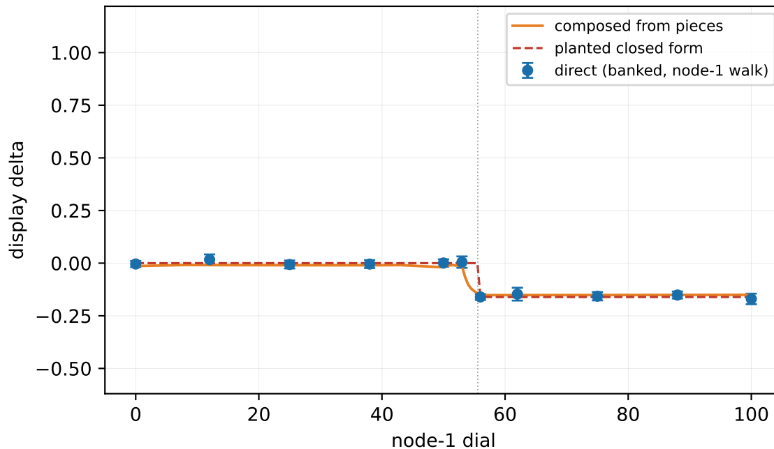
THE REFEREE: node-1 → node-3 through the live relay 11/11 within propagated bars; step -0.158 (planted -0.161); flip bracketed L53-56
