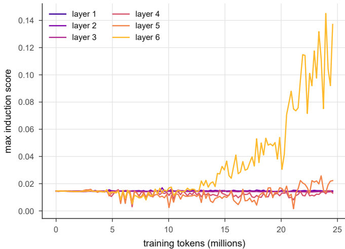
a Induction heads
