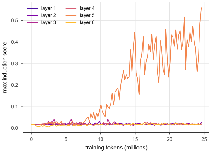
a Induction heads
