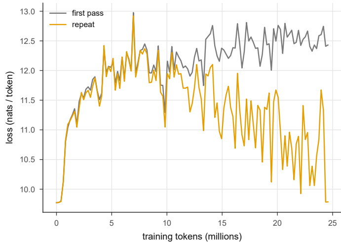
b In-context copying
