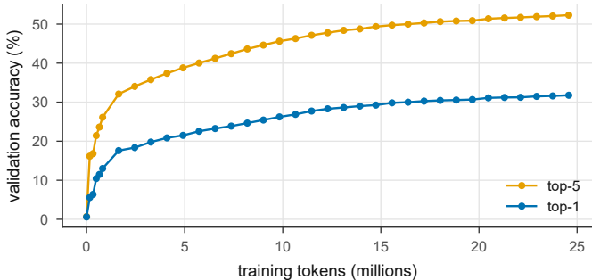
Next-token accuracy
