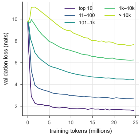
c Loss by token frequency
