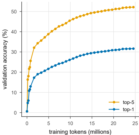
a Next-token accuracy
