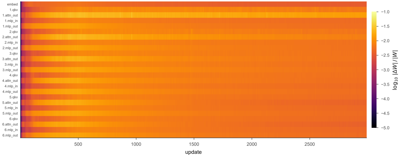
Update size per weight matrix
