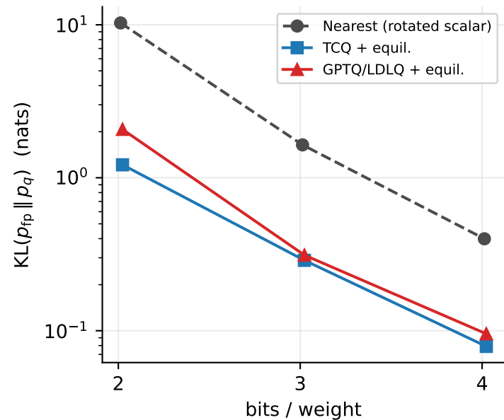
(a) Distortion vs. rate
