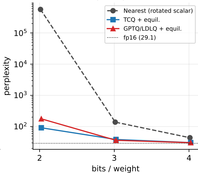
(b) Perplexity vs. rate
