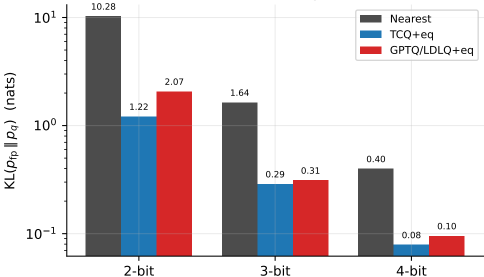
Error feedback and trellis coding vs. nearest rounding
