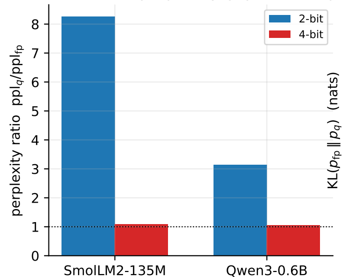
(a) Relative perplexity gap (TCQ+eq)
