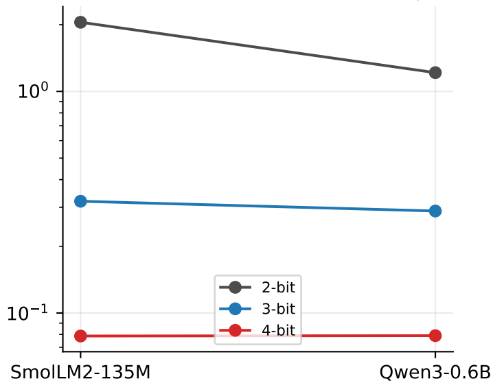
(b) KL vs. model size (TCQ+eq)
