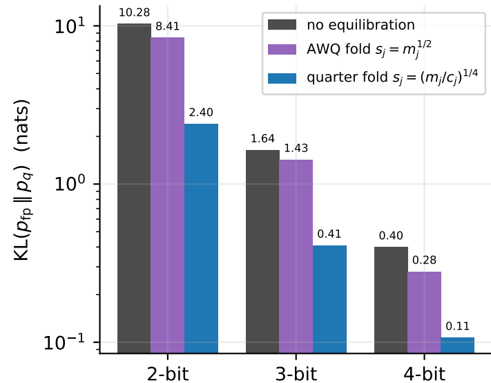
Equilibration exponent ablation (rotated scalar quantizer) Qwen3-0.6B
