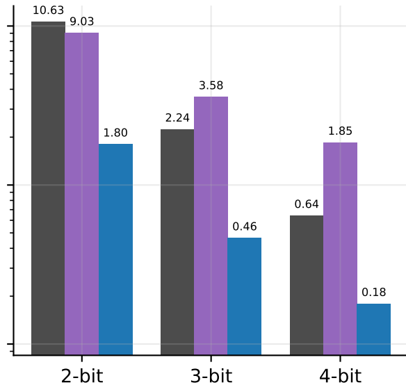
Equilibration exponent ablation (rotated scalar quantizer) Qwen3-0.6B
