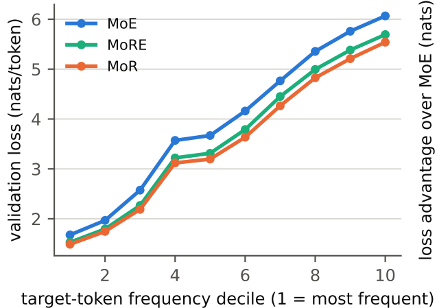
(a) Loss by token difficulty
