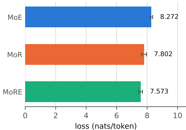
(b) Out-of-domain (the Pile)
