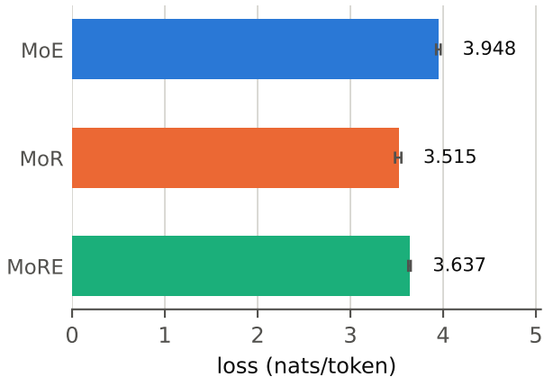
(a) In-domain (WikiText-103 val)
