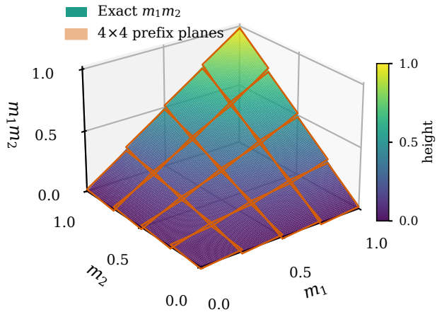
(b) The mantissa product, tiled ( k = 2 )
