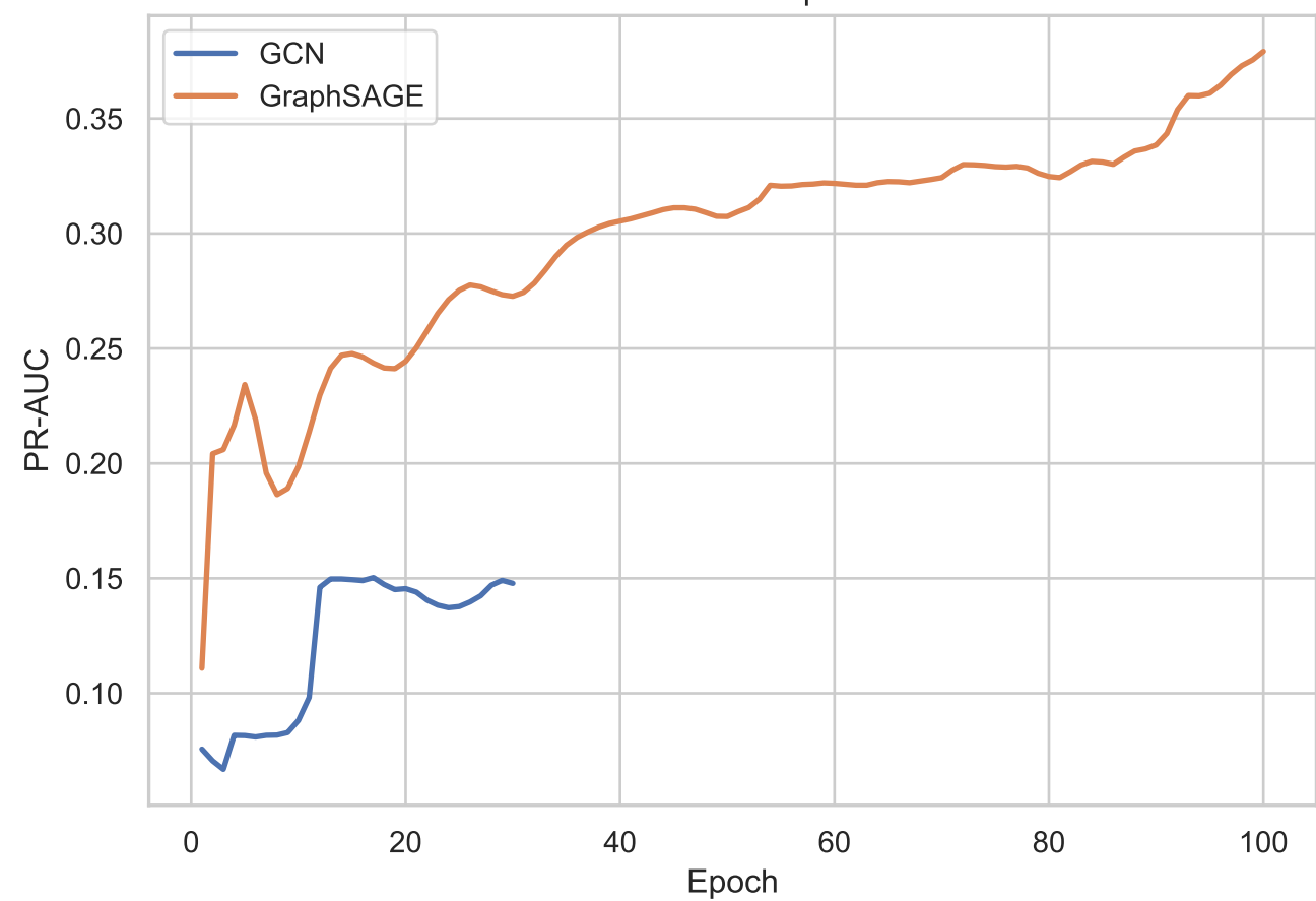
PR-AUC over Epochs
