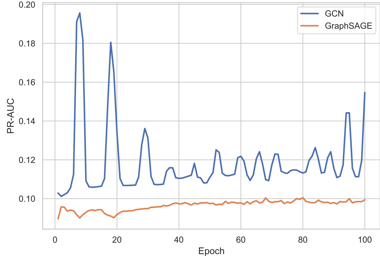
PR-AUC over Epochs
