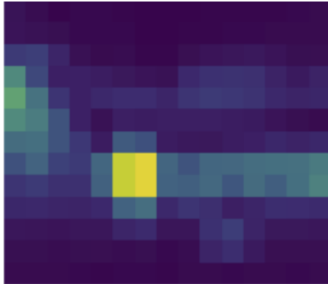
Reconstruction Error
