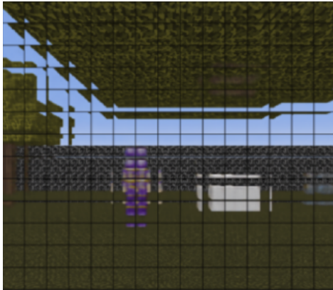
Reconstruction \hat{X}
