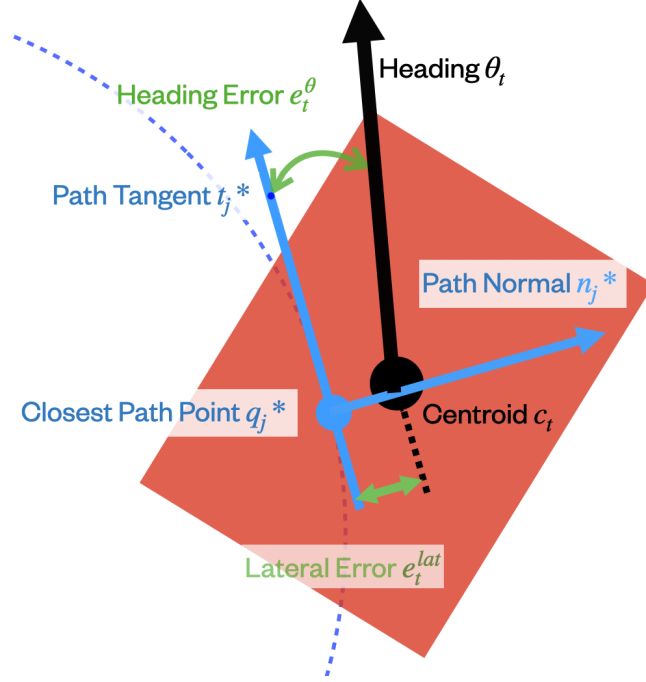
Figure 6.5: Diagrammatic representation of the state space in the parameterized MDP. The object’s pose is represented relative to the reference path through lateral deviation e_t^{\text{lat}} , heading error e_t^\theta , and velocity components along the path tangent and normal. The normalized contact-resistance descriptor z conditions the policy on the interaction regime.
