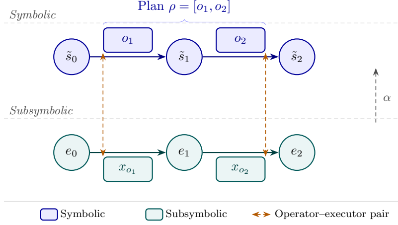
Figure 2.3: The two-level structure of the hybrid planning and learning framework. Top (symbolic): The agent generates a plan \rho as a sequence of operators o_i transitioning between symbolic states \tilde{s} . Bottom (subsymbolic): The environment consists of concrete states e , and transitions are realized by executors x_{o_i} —policies that implement the corresponding operators. The abstraction function \alpha : \mathcal{S} \rightarrow \tilde{\mathcal{S}} maps environment states to symbolic descriptions. Each operator–executor pair (dashed orange) links a symbolic action to its realization in the environment. Novelty manifests when the executor for an operator no longer achieves the intended symbolic transition.
