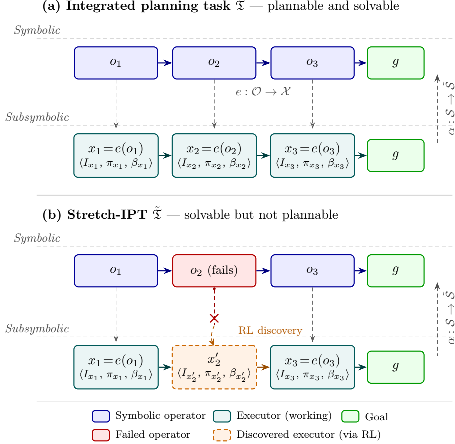
Figure 5.2: Conceptual overview of the integrated planning task (IPT) formalism. Each symbolic operator o_i is mapped to a subsymbolic executor x_i = \langle I_{x_i}, \pi_{x_i}, \beta_{x_i} \rangle via the executor function e . The abstraction function \alpha : \mathcal{S} \rightarrow \hat{\mathcal{S}} maps environment states back to symbolic states for the planner. (a) In a working IPT, all executors realize their associated operators and the agent reaches the goal g . (b) When novelty causes an operator to fail, the IPT becomes a Stretch-IPT: the task remains solvable but the current executor mapping is broken. RAPid-Learn solves the executor discovery problem by constructing a new executor x'_2 through reinforcement learning, restoring solvability.
