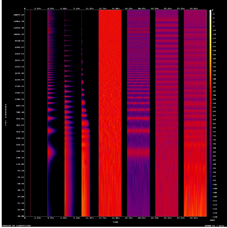
Fig. 1. Comparison spectrogram: click / comb / CQT / evoke CM7, then the same four treatments of noise.
