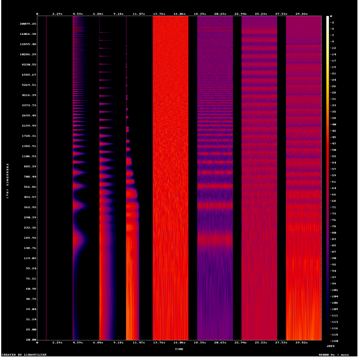
Fig. 1. Log-frequency spectrogram of the comparison sequence (left to right): click; click comb; click constant- Q ; click evoke CM7; noise; noise comb; noise constant- Q ; noise evoke CM7.
