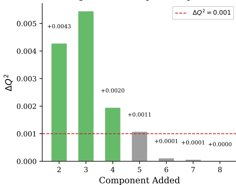
Marginal Q^2 Gain per Component
