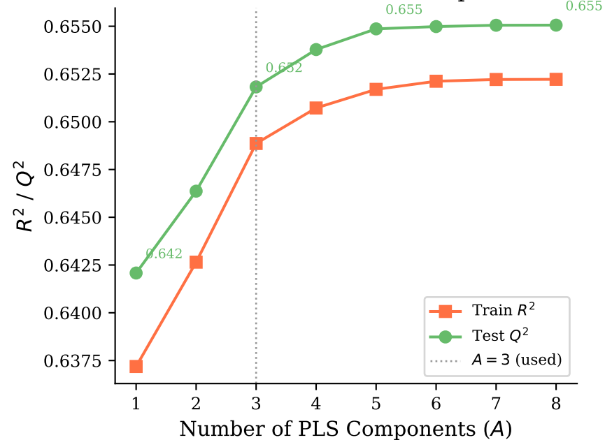
Model Performance vs Components
