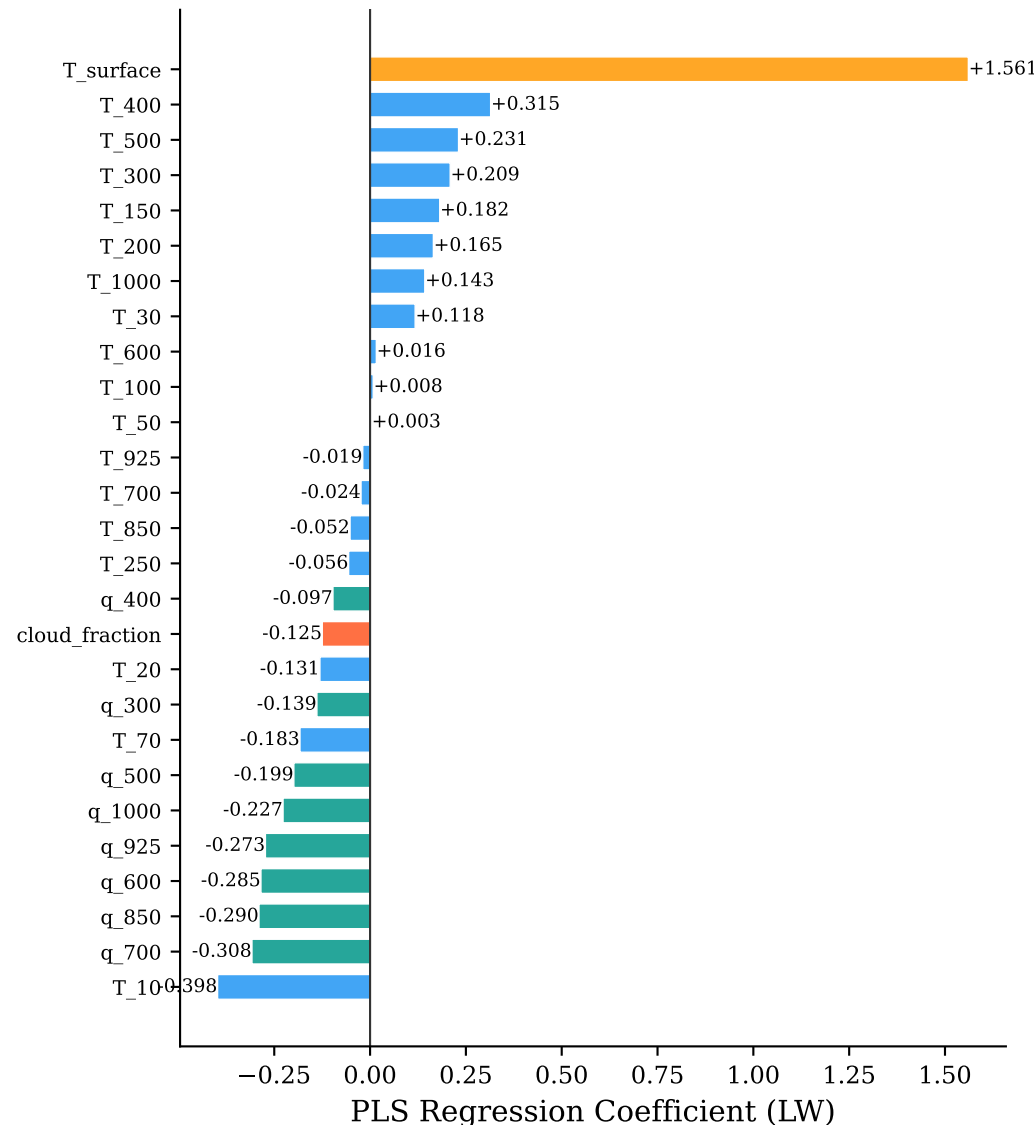
(b) Feature Contributions to \Delta R_{LW}
