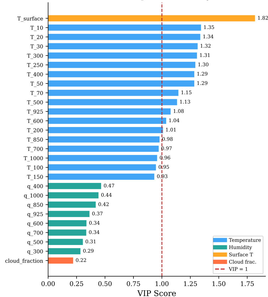
(a) Variable Importance in Projection
