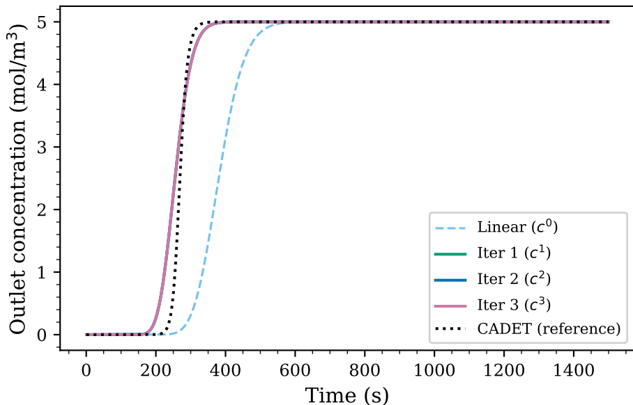
Iteration convergence (Class C Langmuir)
