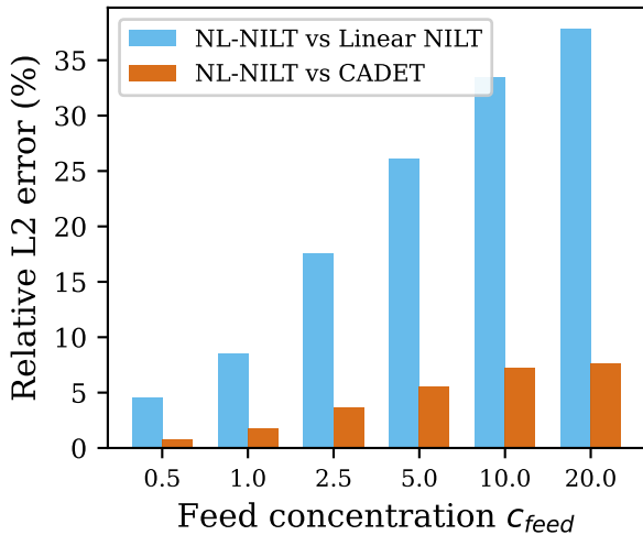
(a) Accuracy
