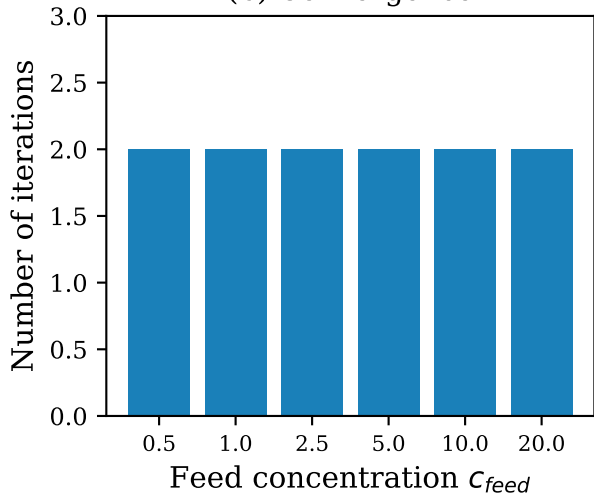
(b) Convergence
