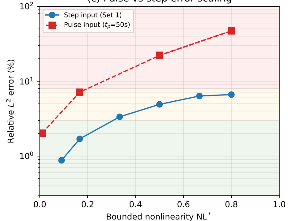
(c) Pulse vs step error scaling
