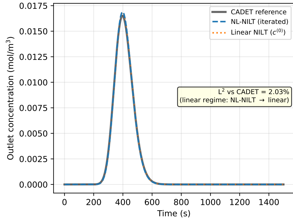
(a) Dilute pulse, linear-limit validation ( c_f=0.05 , NL^*=0.010 )
