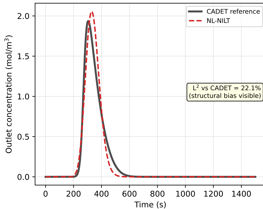
(b) Moderate pulse, peak distortion ( c_f=5.0 , NL^*=0.50 )
