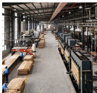
03 Gluing & lay-up
