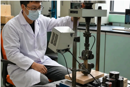
Bonding strength
