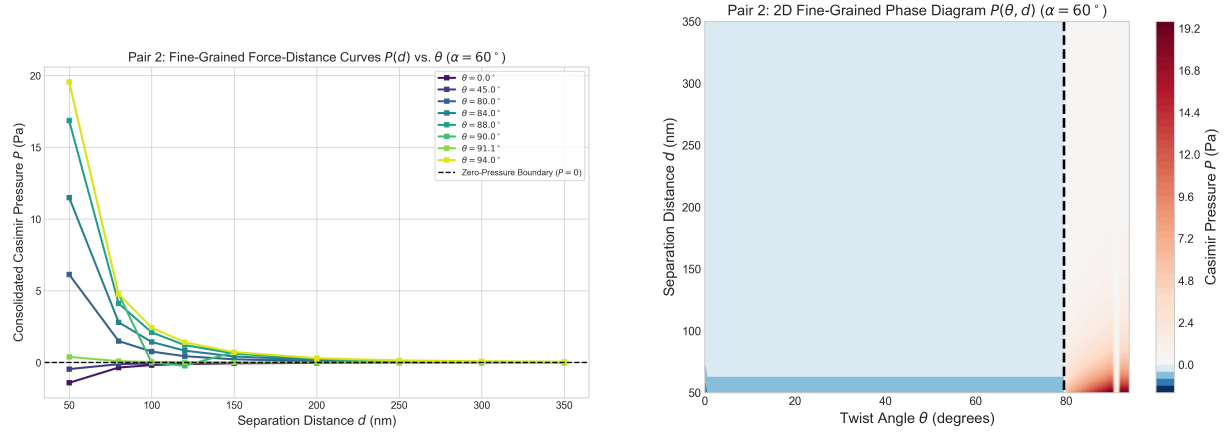
(a) 1D Force-Distance Curves P(d) for various twist angles \theta . (b) 2D Contour Heatmap Phase Diagram P(\theta, d) .
