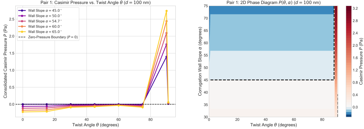
(a) 1D Line Curves P(\theta) for various wall slopes \alpha . (b) 2D Contour Heatmap Phase Diagram P(\theta, \alpha) .
