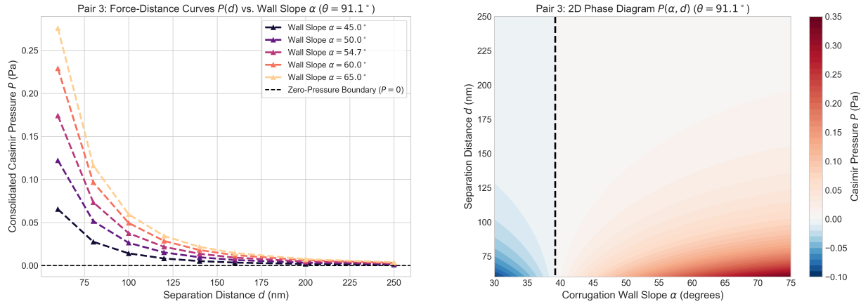
(a) 1D Force-Distance Curves P(d) for various wall slopes (b) 2D Contour Heatmap Phase Diagram P(\alpha, d) .
