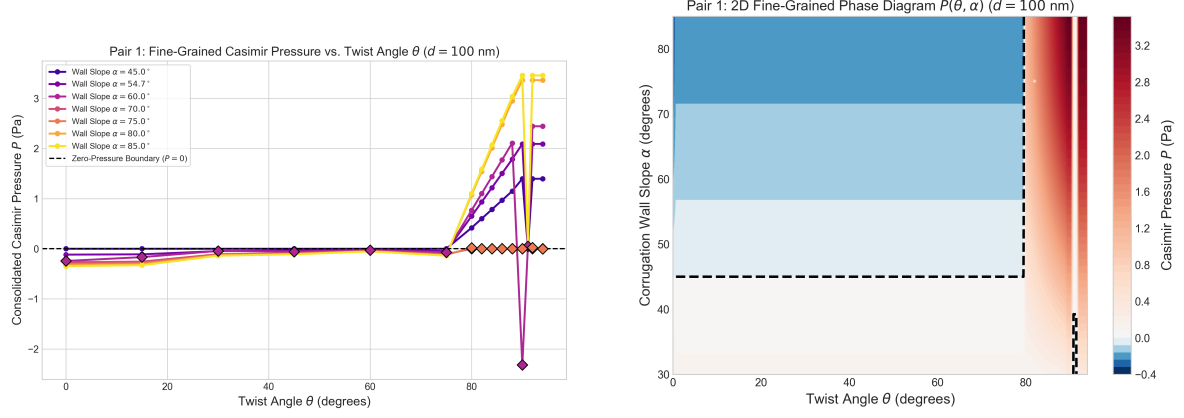
(a) 1D Fine-Grained Line Curves P(\theta) for various wall slopes \alpha at d = 100 nm vs. (b) 2D Fine-Grained Contour Heatmap Phase Diagram P(\theta, \alpha) .
