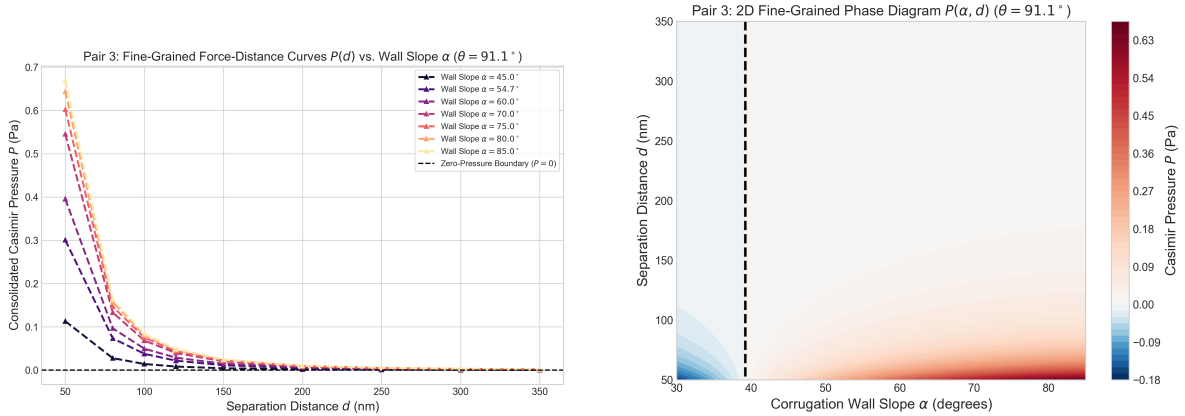
(a) 1D Force-Distance Curves P(d) for various wall slopes \alpha at \theta = 91.1^\circ . (b) 2D Contour Heatmap Phase Diagram P(\alpha, d) .
