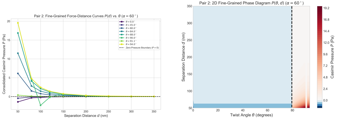
(a) 1D Force-Distance Curves P(d) for various twist angles \theta and (b) 2D Contour Heatmap Phase Diagram P(\theta, d) .
