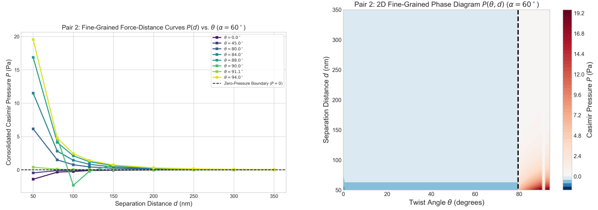
(a) 1D Fine-Grained Force-Distance Curves P(d) for various twist angles \theta at \alpha = 60^\circ vs. (b) 2D Fine-Grained Contour Heatmap Phase Diagram P(\theta, d) .
