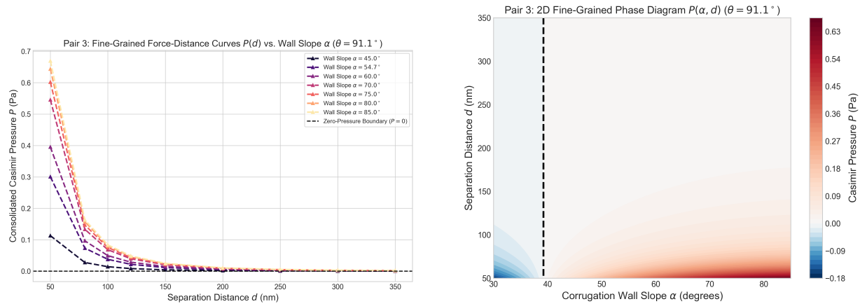
(a) 1D Force-Distance Curves P(d) for various wall slopes \alpha ( \theta = 91.1^\circ ). (b) 2D Contour Heatmap Phase Diagram P(\alpha, d) .
