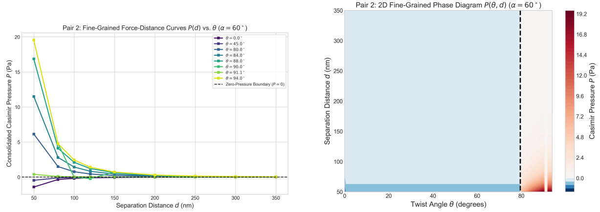
(a) 1D Force-Distance Curves P(d) for various twist angles \theta ( \alpha = 60^\circ ). (b) 2D Contour Heatmap Phase Diagram P(\theta, d) .
