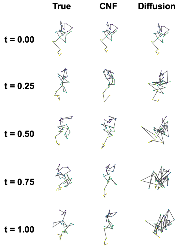
FIG. 4. Placeholder caption for timestep samples from CNF and Diffusion.
