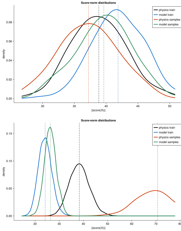
FIG. 2. Placeholder caption for score norm distributions on Rouse base polymers only.
