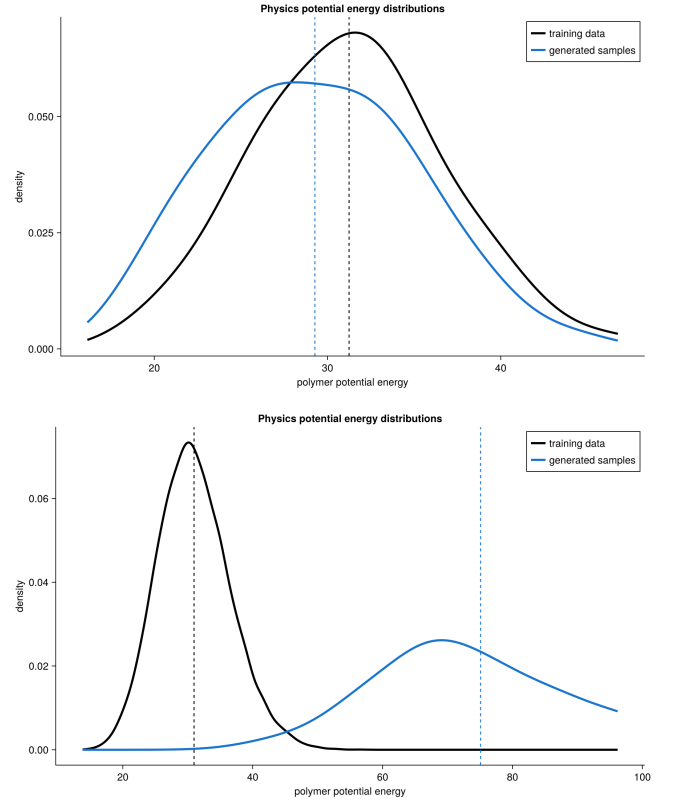
FIG. 3. Placeholder caption for potential energy distributions on Rouse base polymers only.
