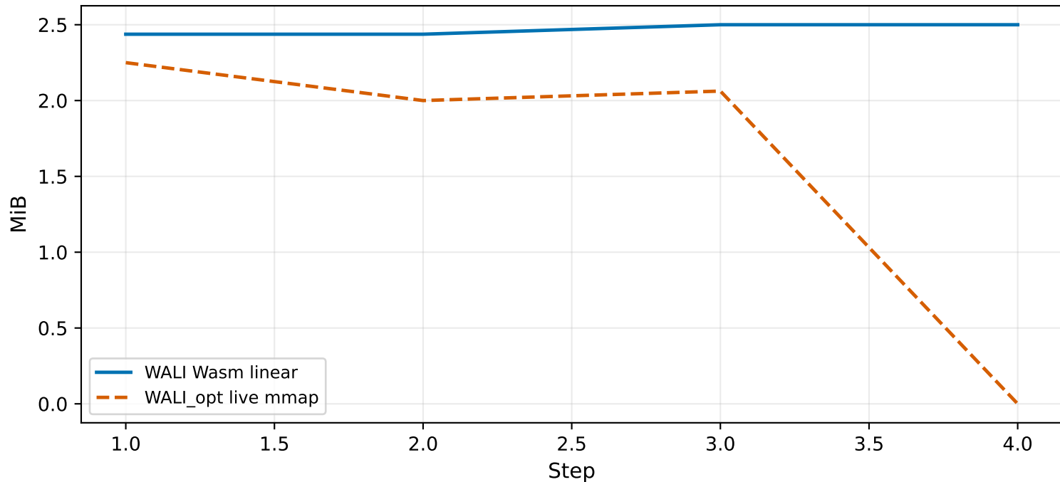
Memory footprint vs step — workload "interleave"
