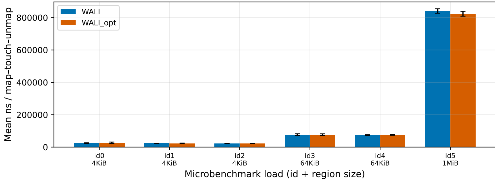
mmap microbenchmark latency
