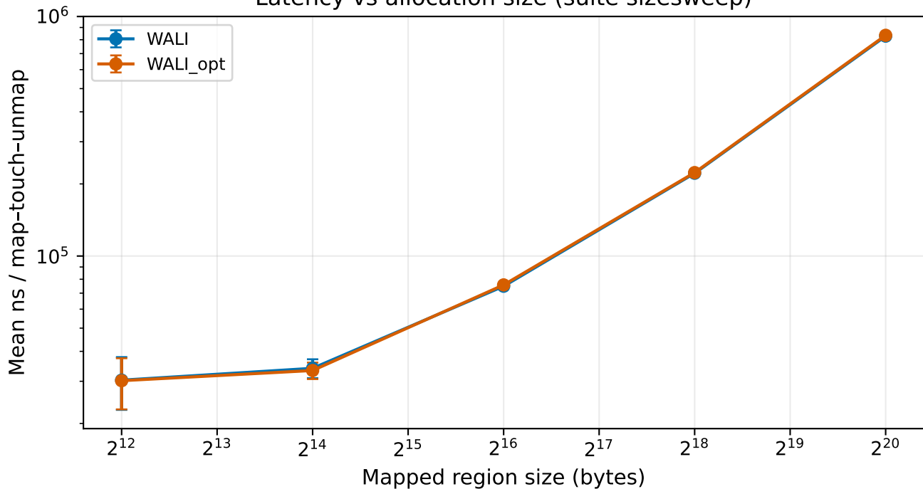
Latency vs allocation size (suite sizesweep)
