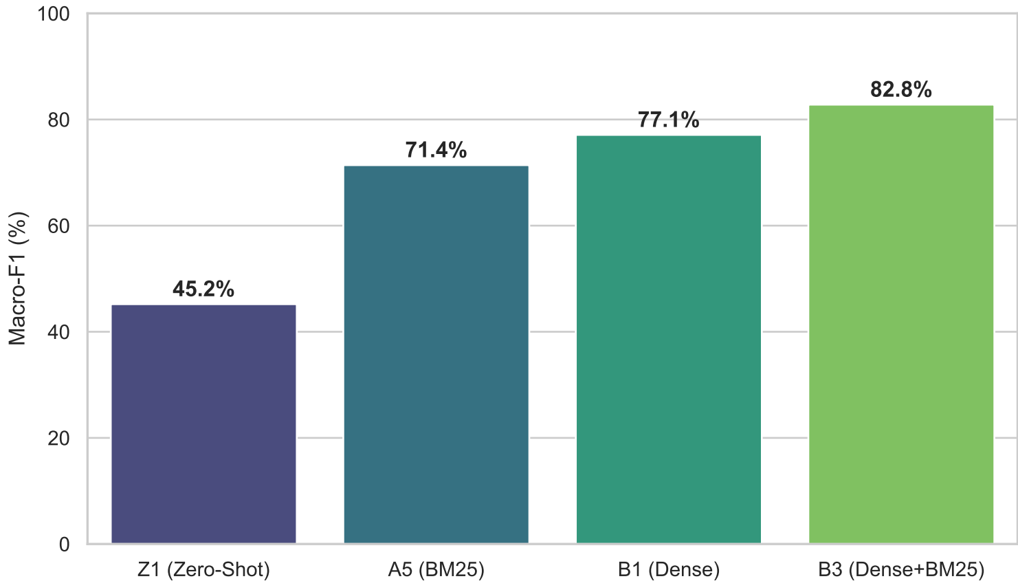
BioASQ: Performance by Configuration
