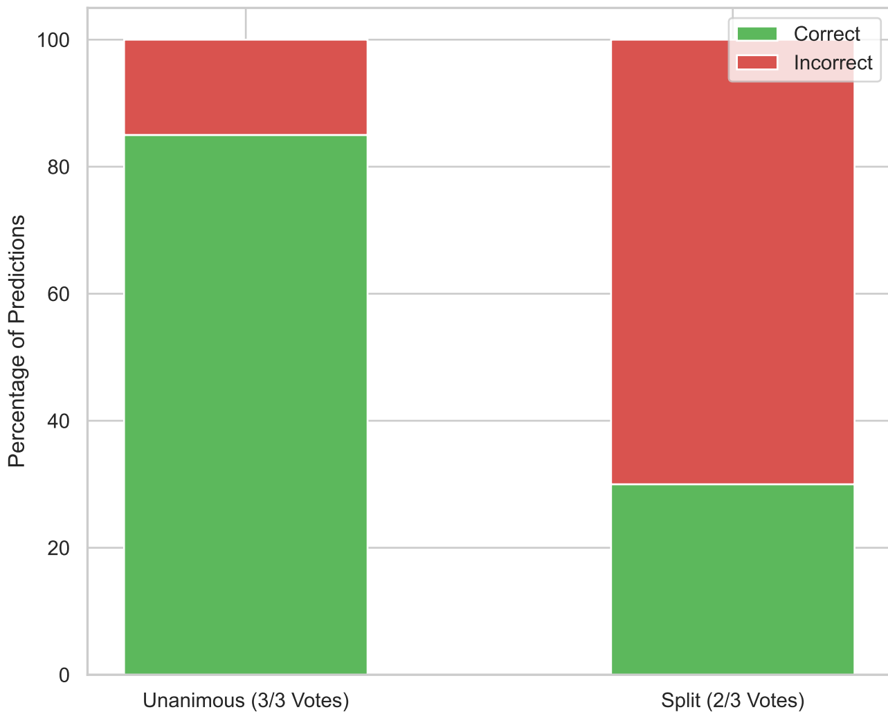
Accuracy by Ensemble Confidence
