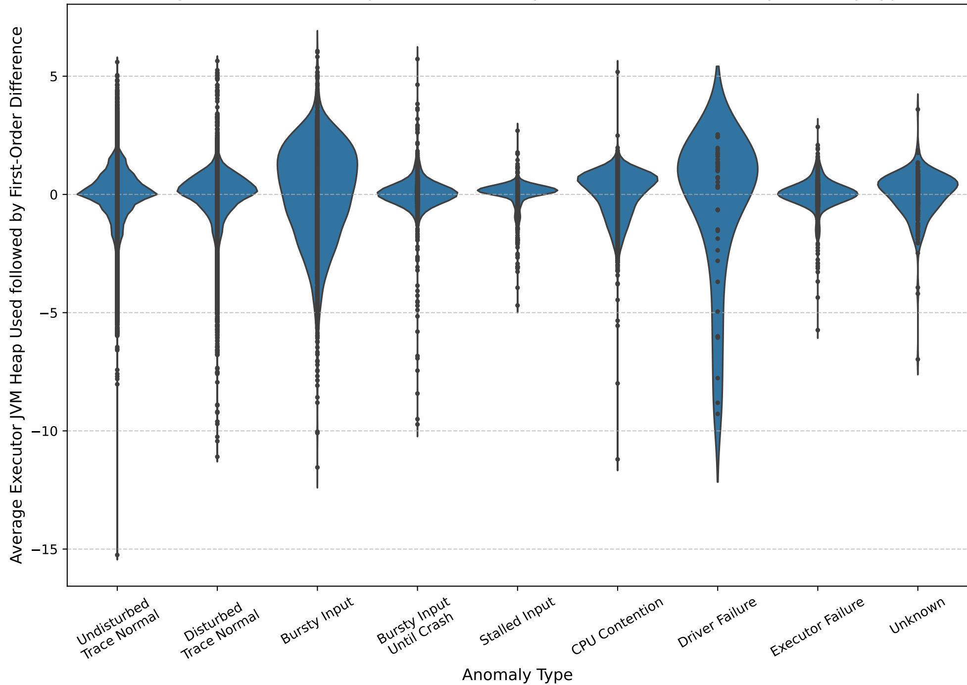
Average Executor JVM Heap Used followed by First-Order Difference by Anomaly Type
