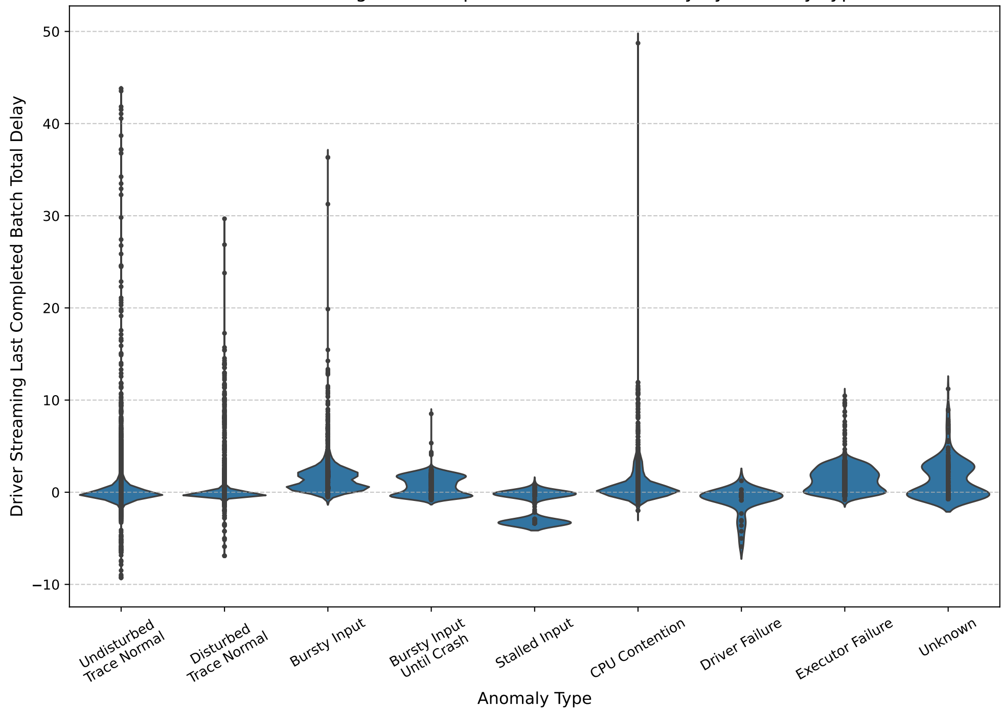
Driver Streaming Last Completed Batch Total Delay by Anomaly Type
