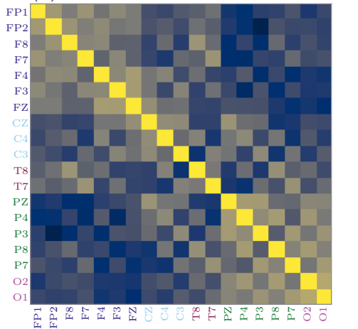
(b) BrainLM-EEG
