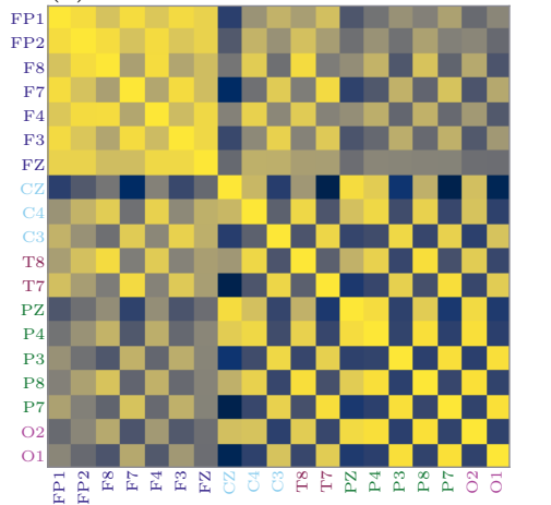
(a) BrainLM-EEG-RoPE
