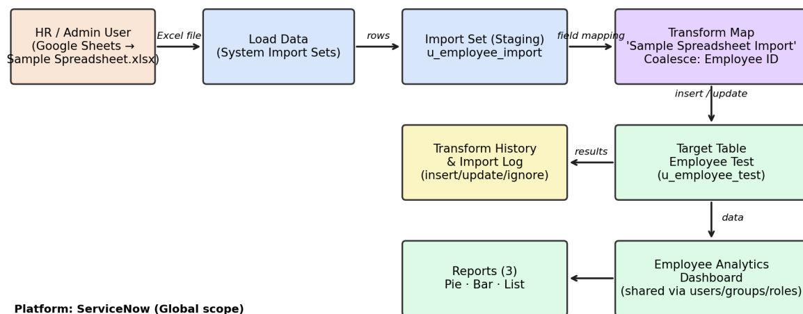
Figure 1: Architecture and data flow of the employee data import, transformation and reporting solution on ServiceNow
