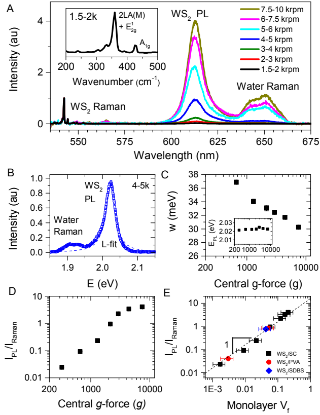
Figure 5: Photoluminescence data for dispersions with different monolayer content. A) Photoluminescence ( \sim 610 nm) and Raman ( \sim 540 nm) spectra of surfactant-stabilized \text{WS}_2 dispersions prepared with different centrifugation conditions and measured in liquid using a Raman spectrometer ( \lambda_{\text{exc}}=532\text{nm} ). The spectra were normalized to the 2LA(M) Raman mode of \text{WS}_2 . The feature at \sim 650 nm is the water Raman peak. Inset: Raman spectrum of dispersed \text{WS}_2 nanosheets plotted versus wavenumber. B) Photoluminescence spectrum of \text{WS}_2 , plotted on an energy scale and fitted to a Lorentzian. C) PL linewidth, from Lorentzian fit, plotted versus central centrifugation acceleration (expressed in units of g). Inset: PL position vs. g-force. D) Ratio of PL intensity to Raman intensity, I_{\text{PL}}/I_{\text{Raman}} , plotted vs. g-force. E) I_{\text{PL}}/I_{\text{Raman}} plotted versus monolayer volume fraction. The dashed line represents I_{\text{PL}} / I_{\text{Raman}} = 17 \times V_f .
