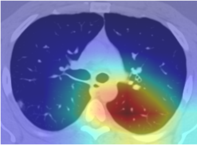
CT Segmentation
