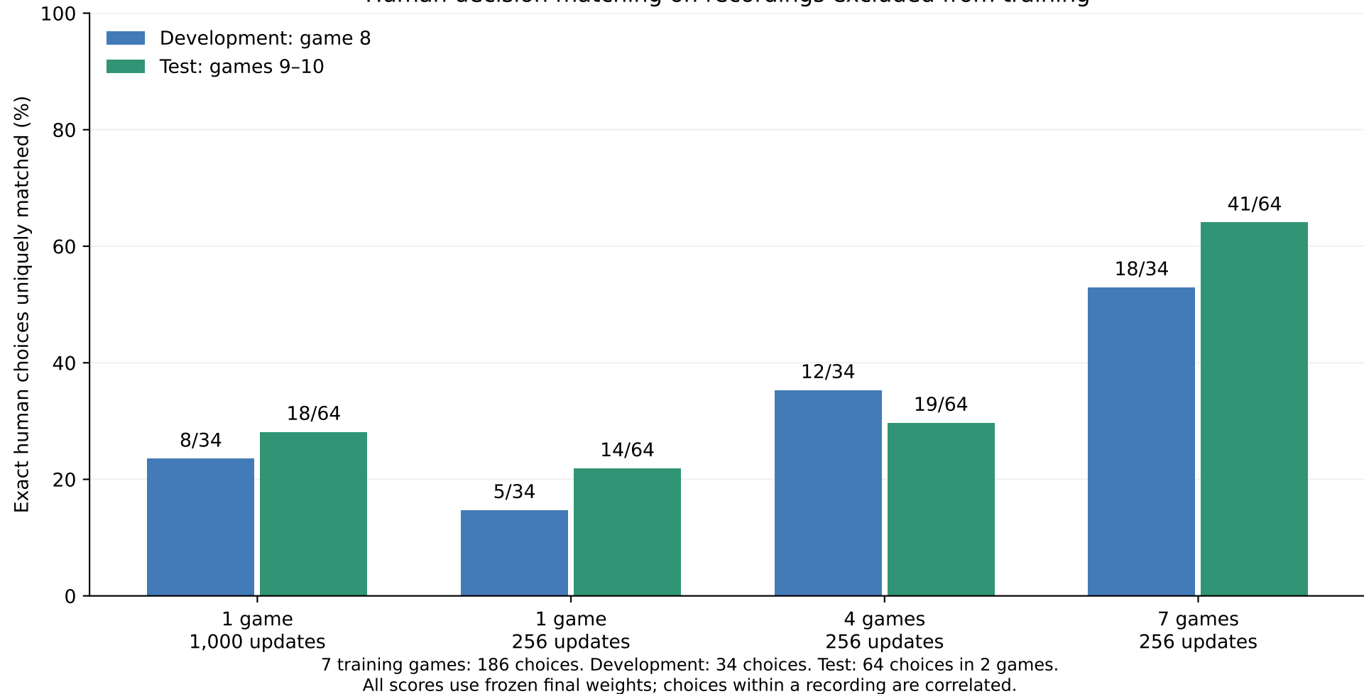
Human decision matching on recordings excluded from training
