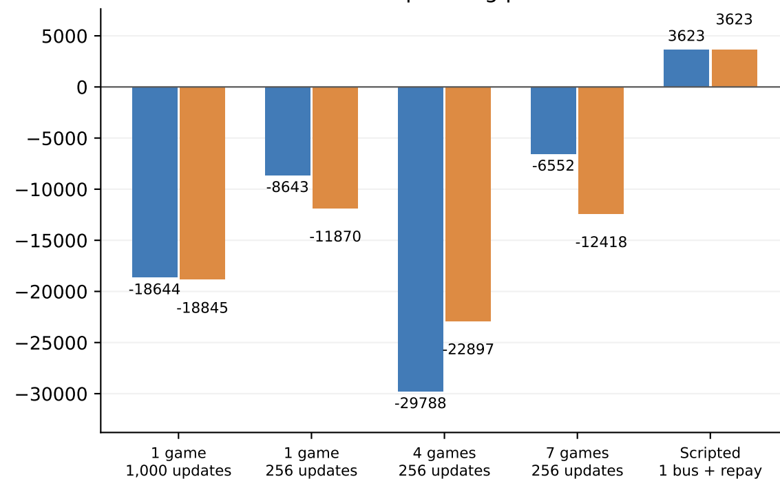
Sustained profitable passenger service (episodes / 25)
