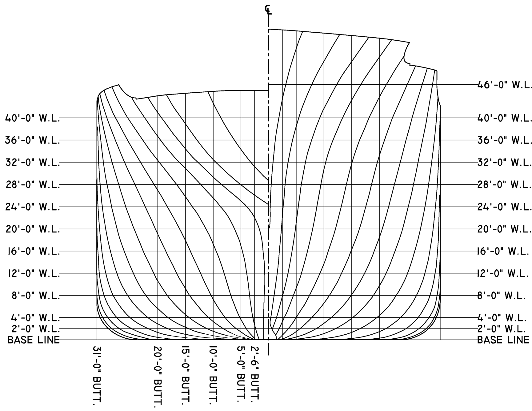
BODY PLAN
