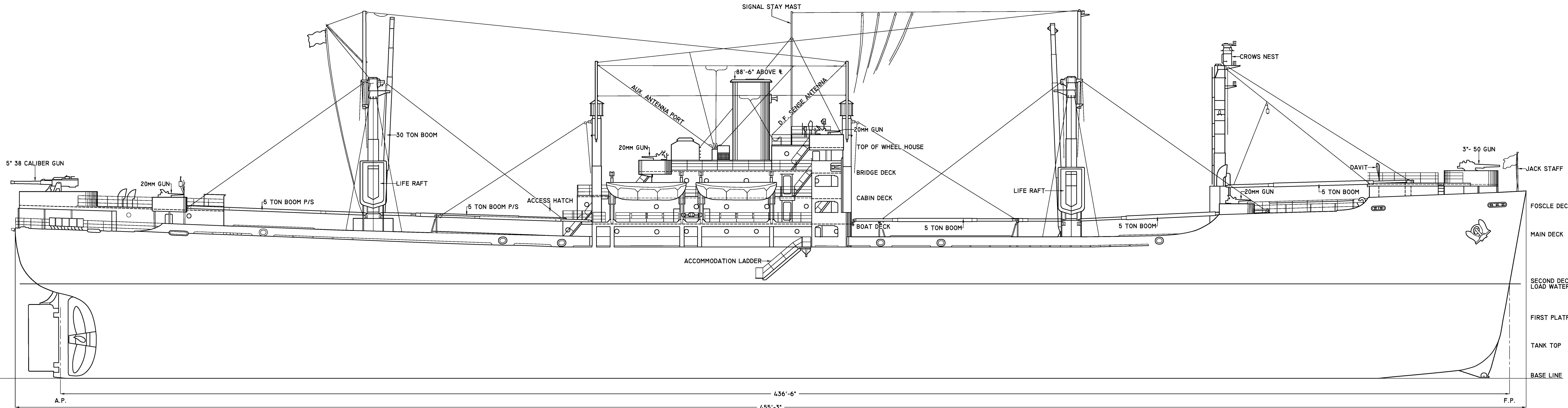
OUTBOARD PROFILE
