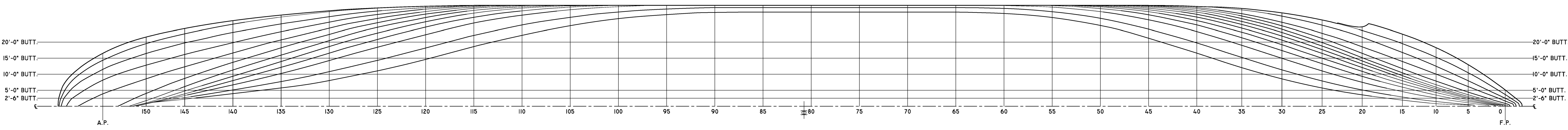
HALF-BREADTH PLAN
