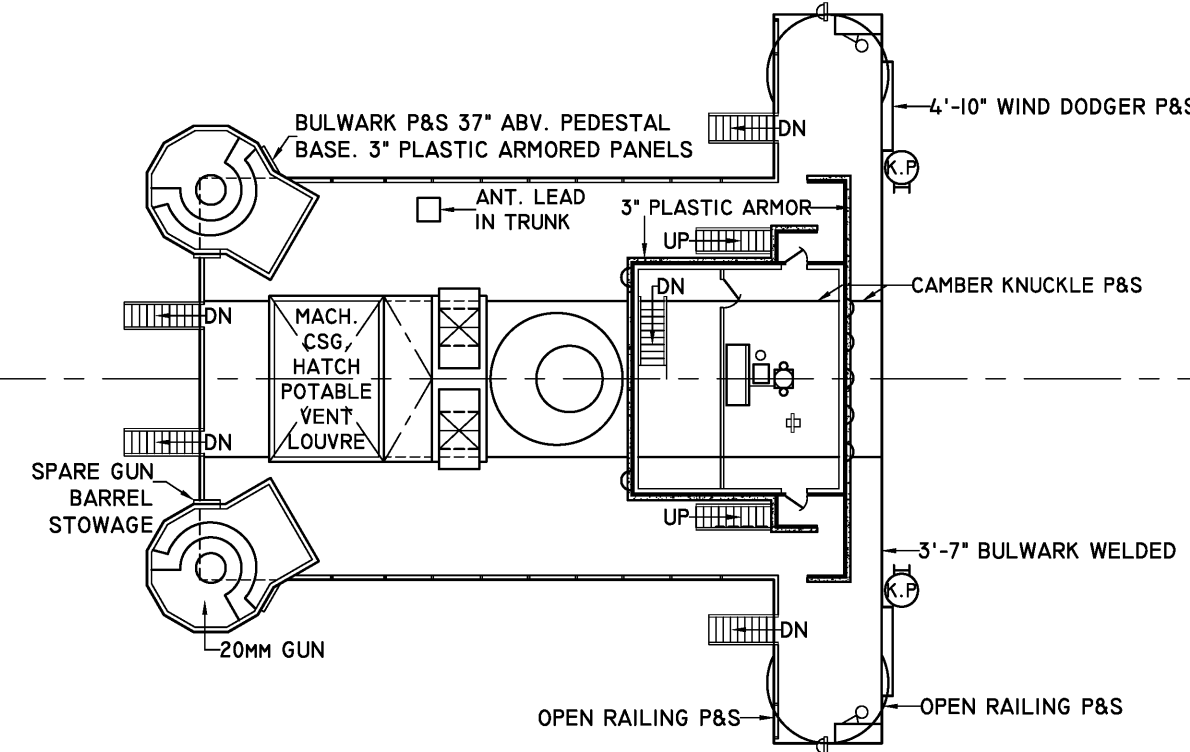
BRIDGE DECK
