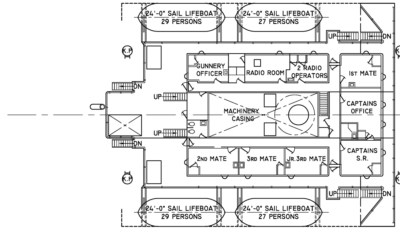
CABIN DECK
