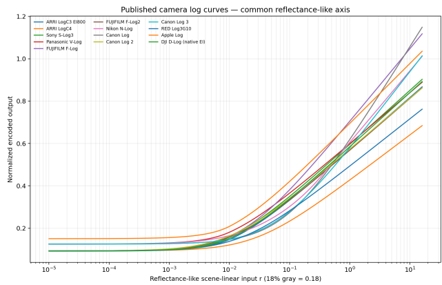
scene-linear: curve
