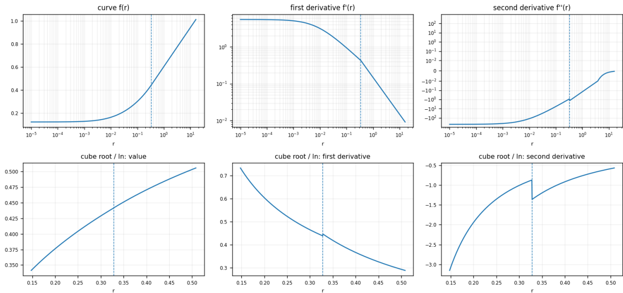
Nikon N-Log
