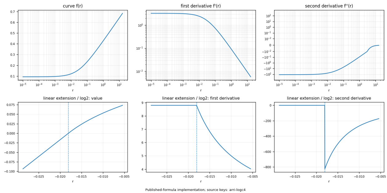
ARRI LogC4
