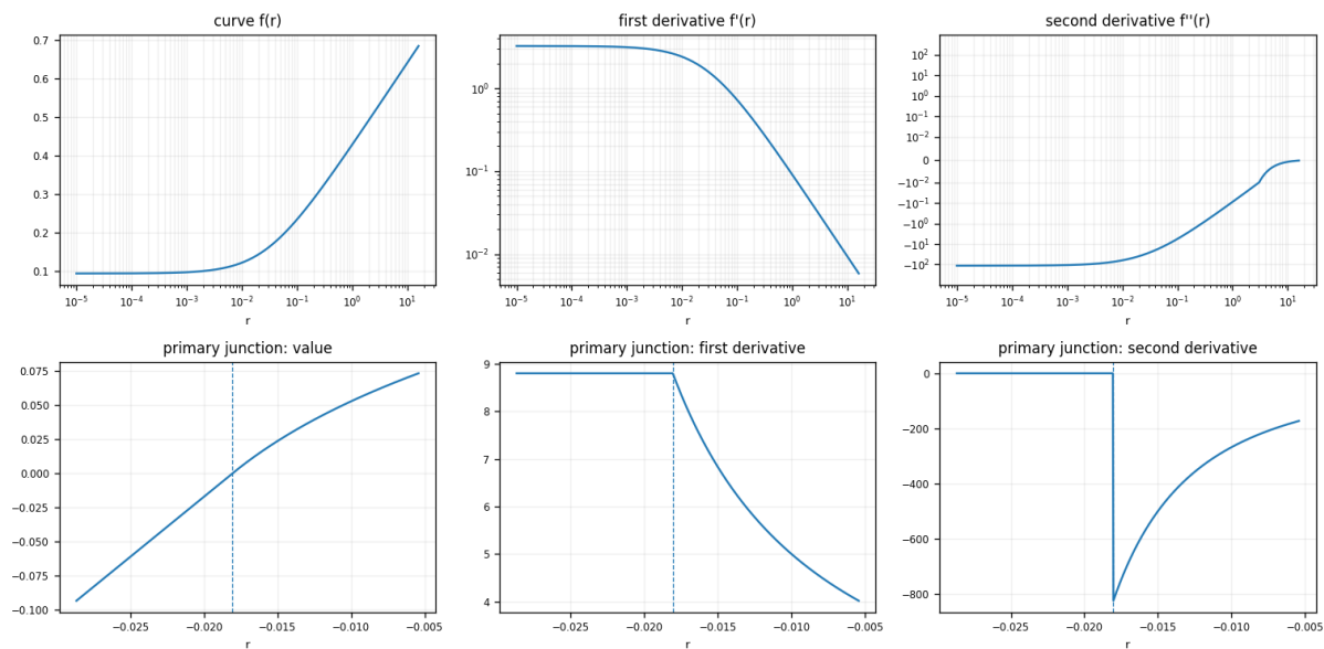
ARRI LogC4
