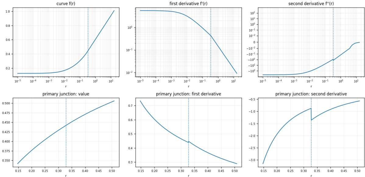
Nikon N-Log
