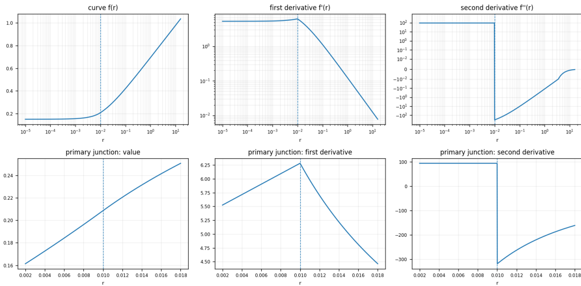
Apple Log
