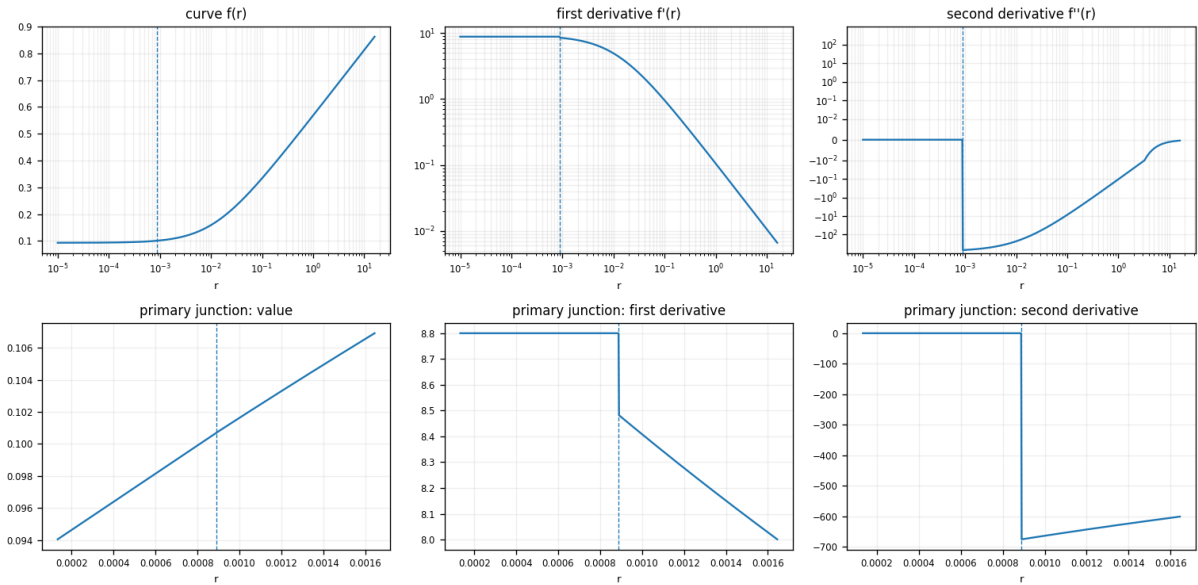
FUJIFILM F-Log2
