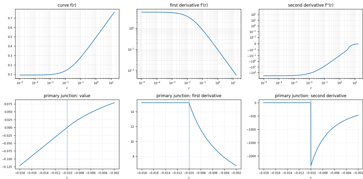
RED Log3G10
