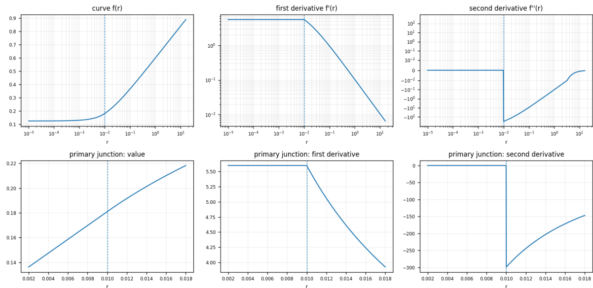
Panasonic V-Log
