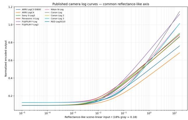
scene-linear: curve
