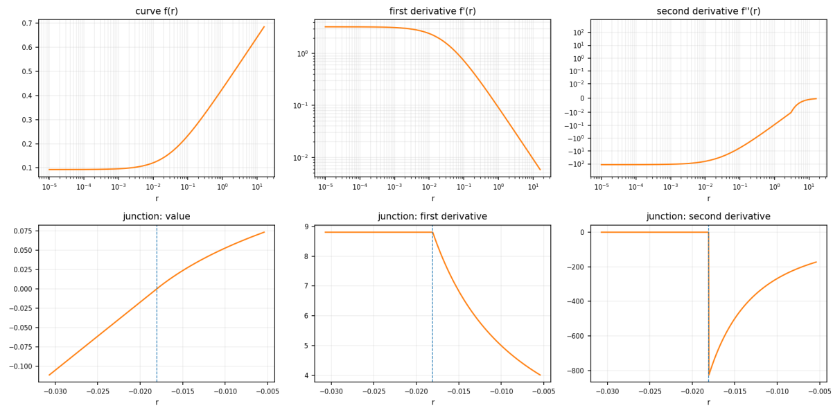
ARRI LogC4
