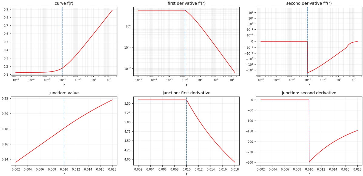
Panasonic V-Log
