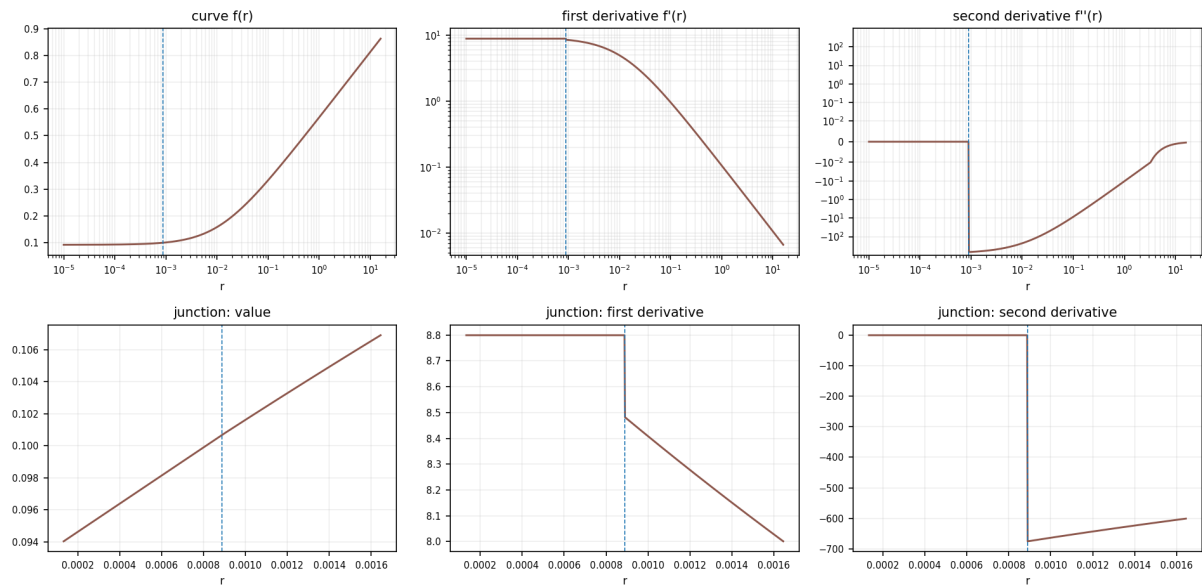
FUJIFILM F-Log2
