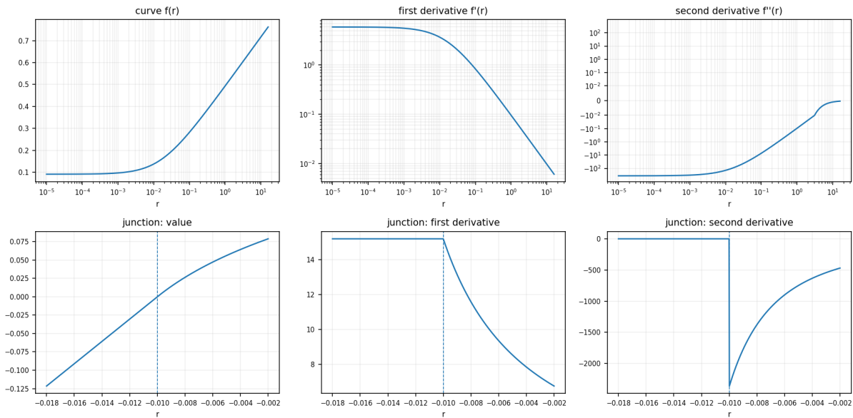
RED Log3G10
