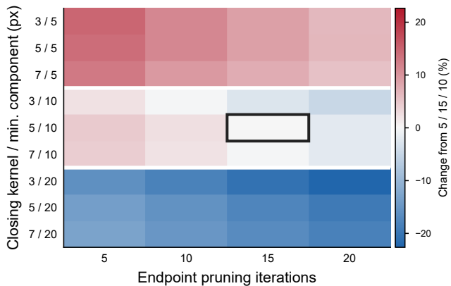
a Retained segments: Annotation-mask mean
