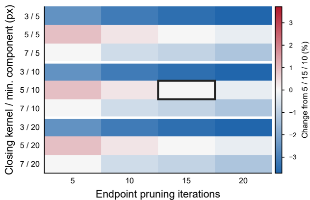
c Junction regions: Annotation-mask mean
