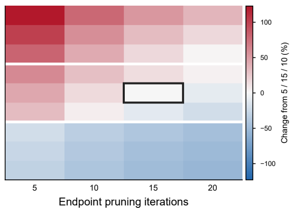
b Retained segments: Matched OOF MAE
