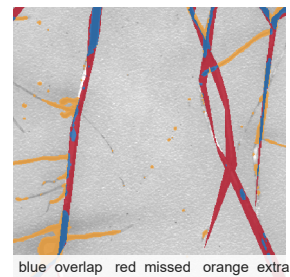
Prediction errors
